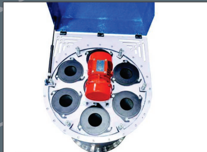
RMC Silo Vent Filter Cartridge
